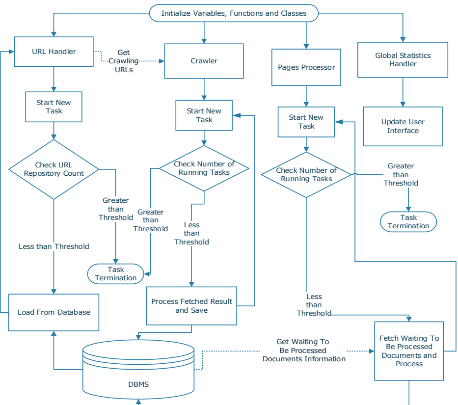
Figure 1: Flowchart of EcCrawler
